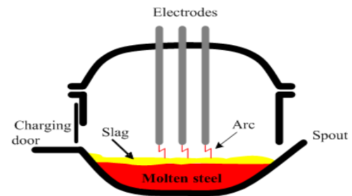
Electric Arc Furnace ( high voltage heating)
